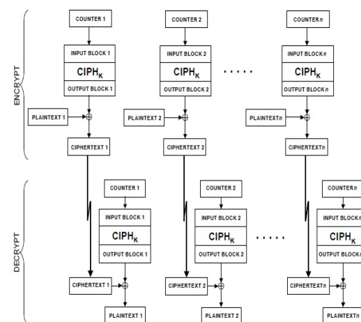
図2: Counter Mode
