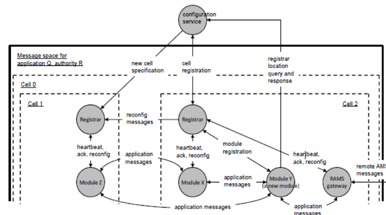
図1: Architectural Elements of AMS (a Single Continuum)
