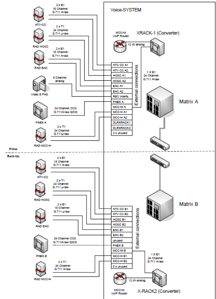
図2: MCC (Matrix A) - MCC (Matrix B) 間の接続例
